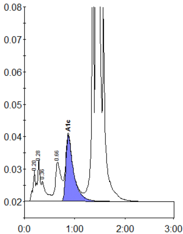
Peak table - ID: 10347339
